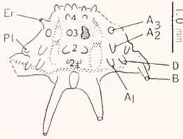
Figure 10. Xanionurus boucati n. gen., n. sp. Major paired spines of small cranium, original of Plate 18, figures 8, 9, 11, 12. Spines lettered as in Figure 9.
